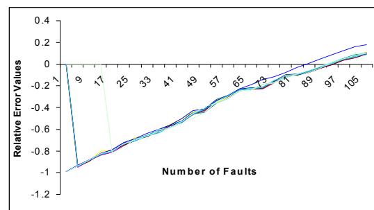
Figure 3. Median relative error values for different fault counts for artifact B
