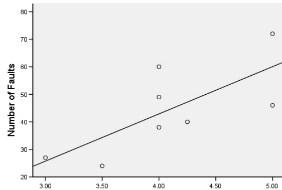
Figure 6. Process Conformance vs. Effectiveness
